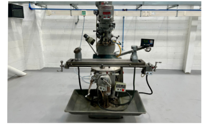
29815 BRIDGEPORT Series 1 2HP Variable Speed Turret Mill with Slotting Attachment and DRO.
