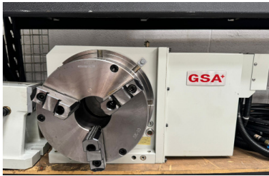
29899 UNUSED GSA 320R Hydraulic 4th Axis and Tailstock. 10" Chuck. Year 2020
