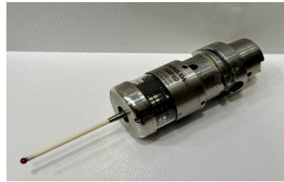
29908 RENISHAW OMP 60 Machine Tool Probe
