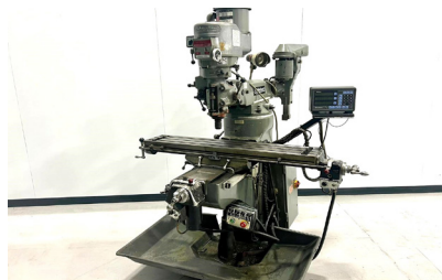
29488 BRIDGEPORT Series 1 2HP Turret Milling Machine with Slotting Attachment and Mitutoyo DRO
