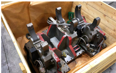
28730 3 x ATLING Model LZB 100-310 Hydraulic Steadies with Hydraulic Pack (Previously used on a Bed Milling Machine). Year 2012
