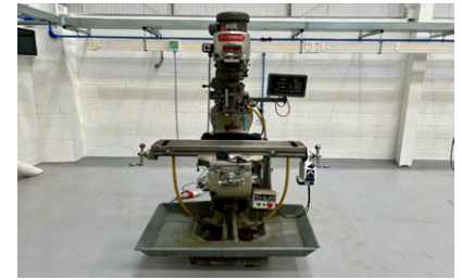
29814 BRIDGEPORT Series 1 2HP Variable Speed Turret Mill with DRO
