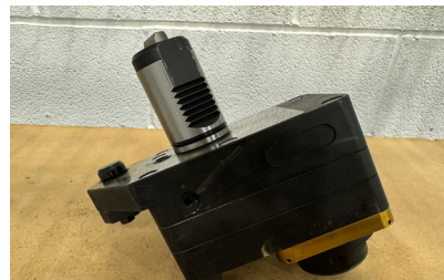
29883 MAZAK Axial Driven Tool Holder. VDI 40
