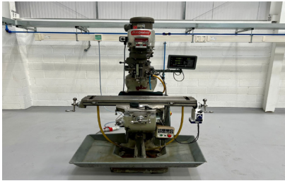
29814 BRIDGEPORT Series 1 2HP Variable Speed Turret Mill with Newall Topaz 2 Axis DRO. Year 1987
