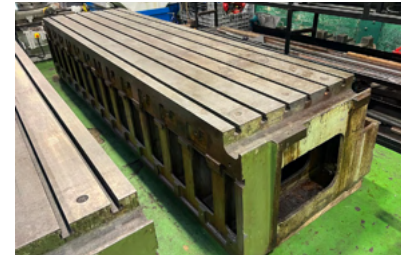
29927 CAST IRON Boxtable 3810mm x 1092mm x 812mm. Weight 6.5 tons
