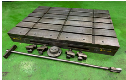
30215 DEVLIEG Rotary T Slotted Sub Table
